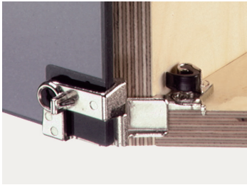
30° Negative angle
