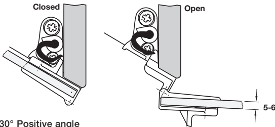
30° Positive angle
