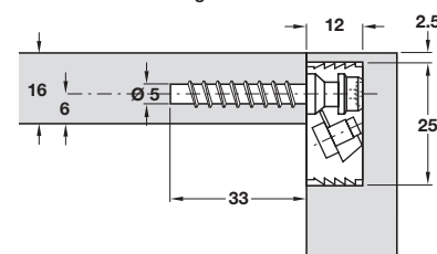
Recommended drilling for 16 mm board thickness
