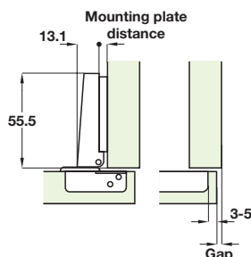
Drilling pattern 48/6
