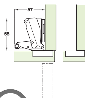
Drilling pattern 48/6
