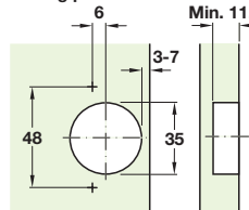
Drilling dimensions for cup fixing Drilling pattern 48/6
