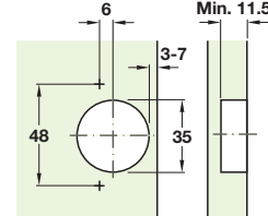
Drilling dimensions for cup fixing Drilling pattern 48/6
