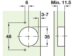
Drilling dimensions for cup fixing Drilling pattern 48/6
