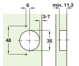
Drilling pattern 48/6
