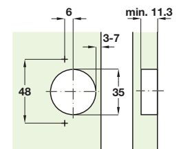
Drilling pattern 48/6
