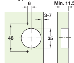
Drilling dimensions for cup fixing Drilling pattern 48/6
