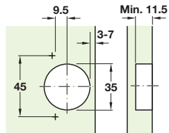
Drilling dimensions for cup fixing Drilling pattern 45/9.5
