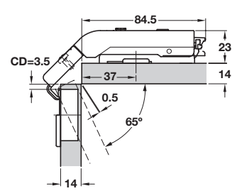
Mounting plate height 0 mm
