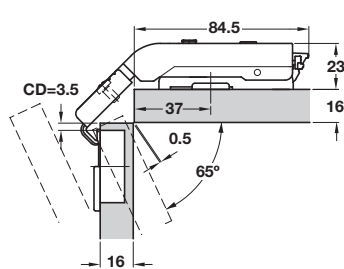
Mounting plate height 0 mm
