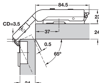
Mounting plate height 0 mm
